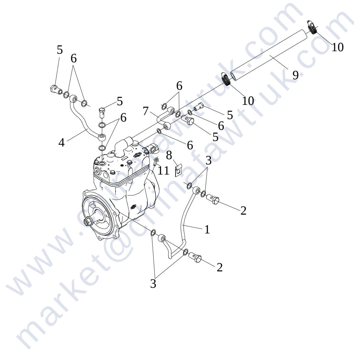
Fig. 37 Air compressor (II)
