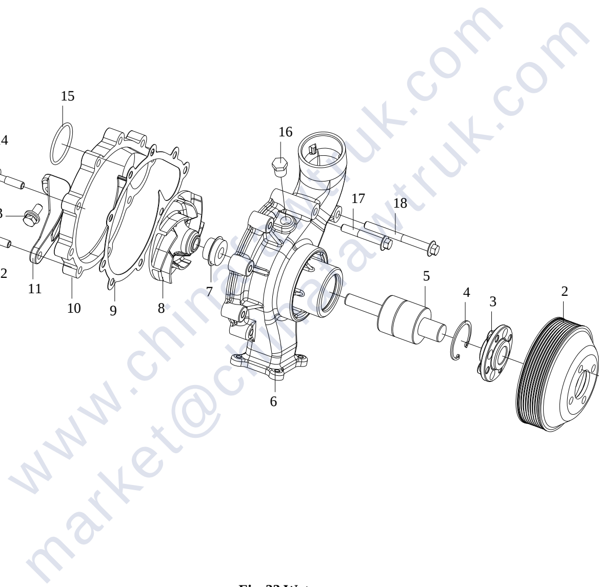
Fig. 33 Water pump
